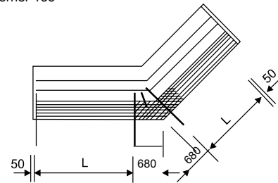
4) Closed corner 135°
