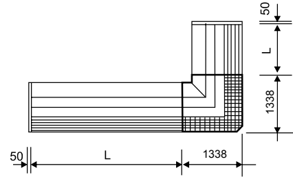
2) Closed corner 90°
