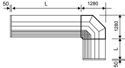
1) Open corner 90°
